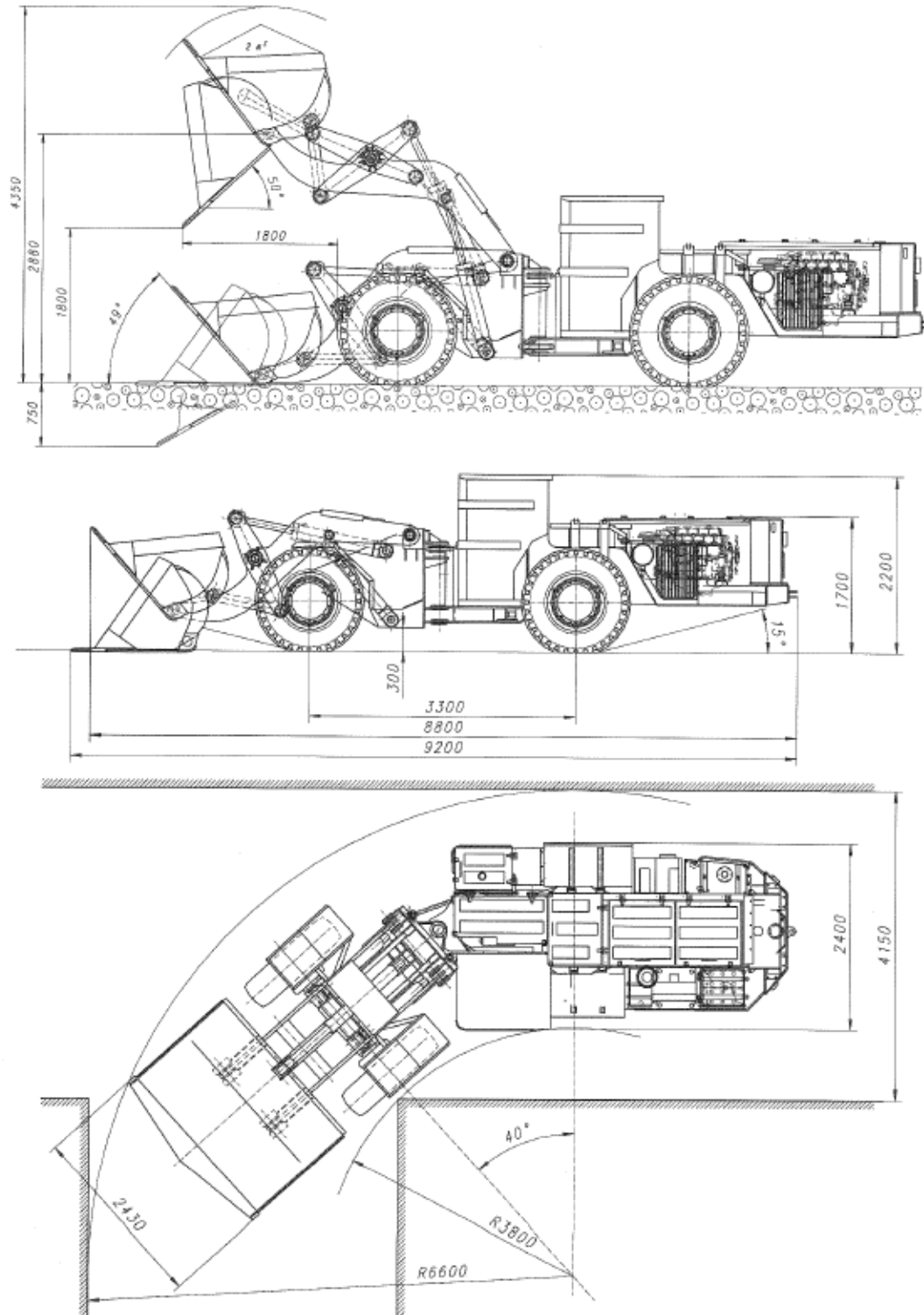
Fig. 1. Loading machine of LKP-0402 type – basic dimensions and parameters
